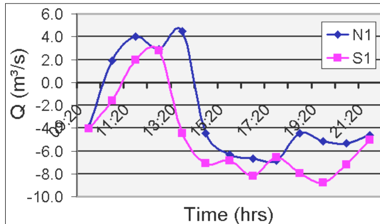
Figure 5. Flow in and out at both mouths (N1, S1) of canal
