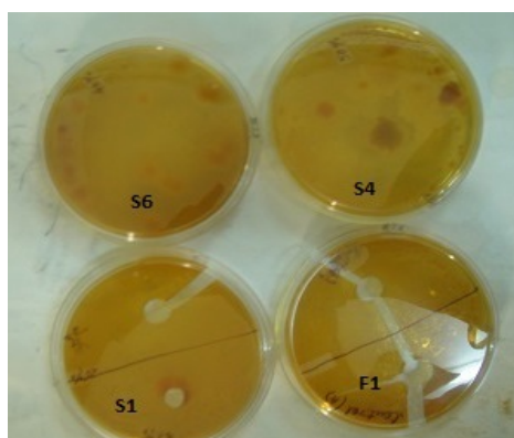
Figure 4. Result of E.coli test
