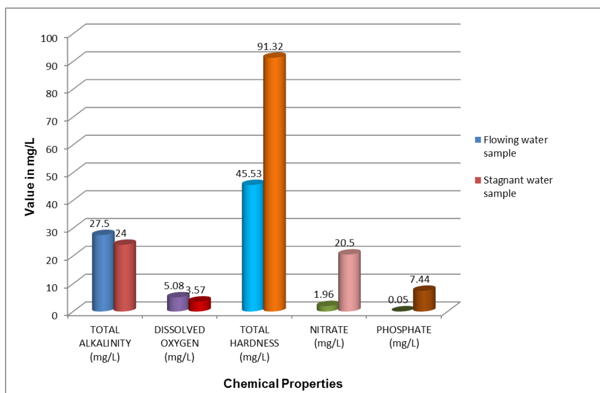
Figure 3. Comparative result of chemical properties of water in flowing and stagnant water samples
