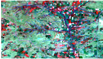
FIG. 1 STUDY AREA ON SATELLITE IMAGERY
