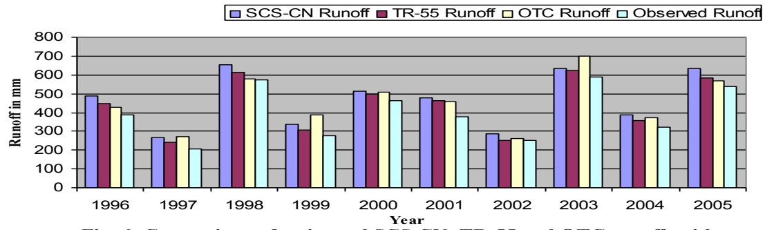
Fig. 6 Comparison of estimated SCS-CN, TR-55 and OTC runoffs with yearly observed runoff
