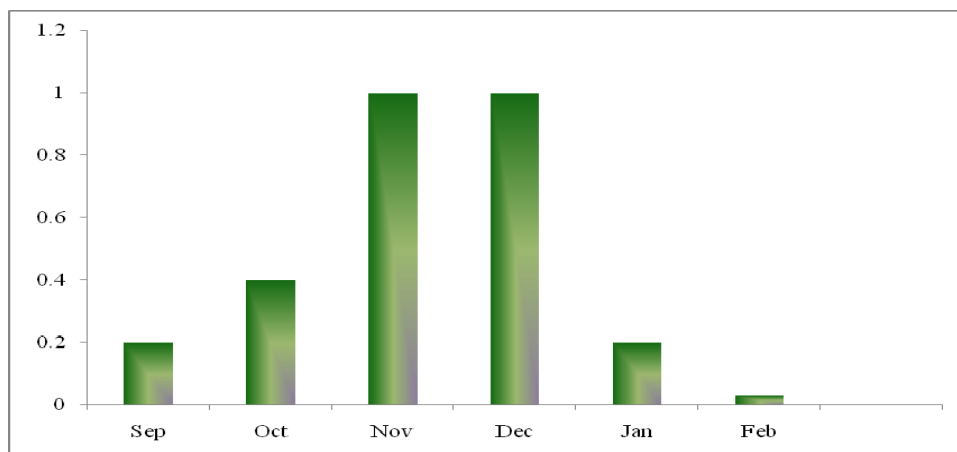
Fig 4. Adequacy Index (PIA) of 4(L) distributory for Zone-A in 2006
