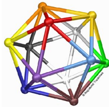
Figure 4. Icosahedron
