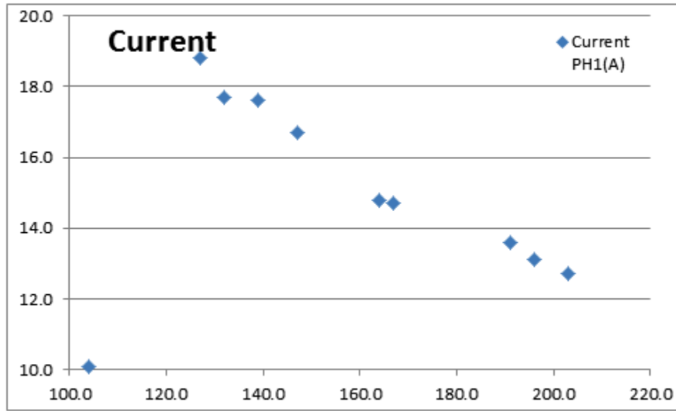
Figure 2. Impact of voltage on motor current, from village Asmadpur Charoli, 24-hour period
